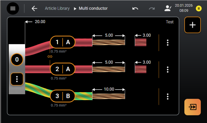
Multiconductors displayed visually and clearly (from «Plus»)
